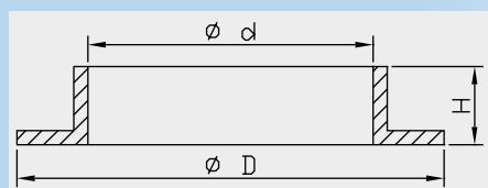
Spring Seat Against Top Cap Steel dimensions
